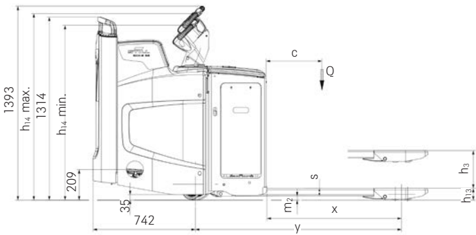
Side view side entry EXH-S
