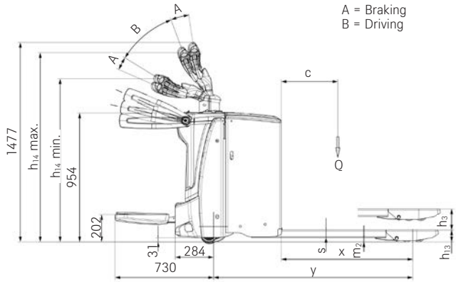
Side view EXH-SF
