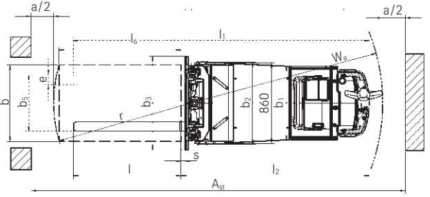
Top view EXV-CB
